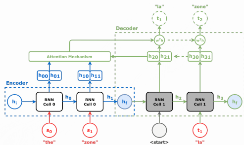
Seq2Seq and Attention Architecture
